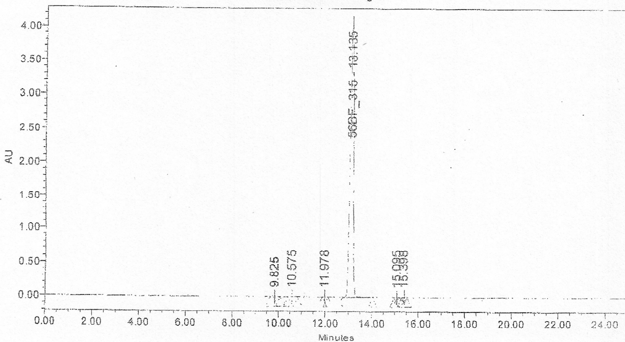
Auto-Scaled Chromatogram
